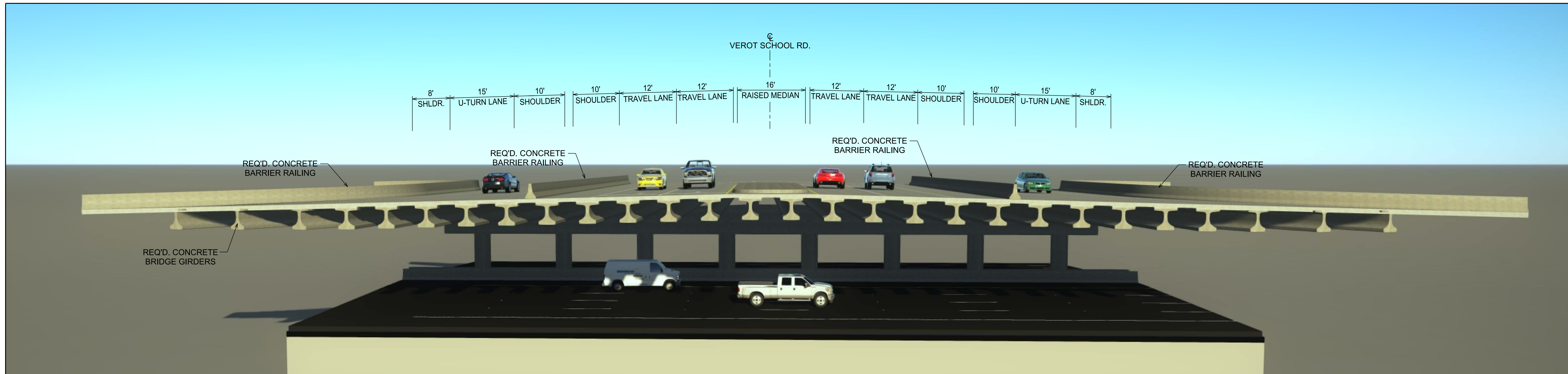
SECTION C-C (LOOKING EAST) VEROT SCHOOL RD. OVER I-49
